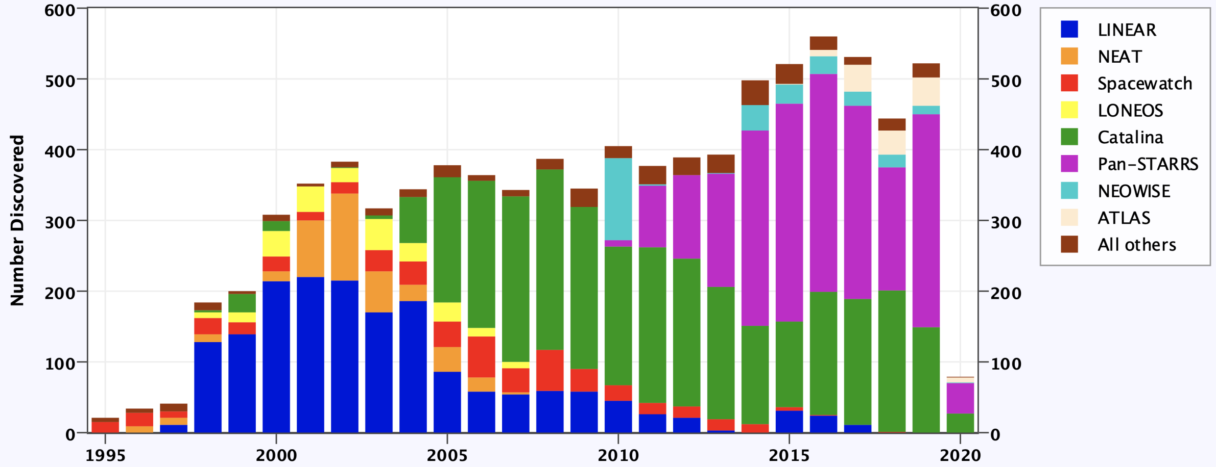
Near-Earth Asteroid Discoveries by Survey ~140m and larger NEAs (as of 2020-Feb-03)
